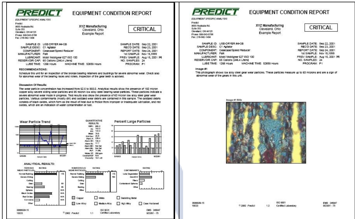
Fig 4. Oil Analysis and Ferroglyphic report.
