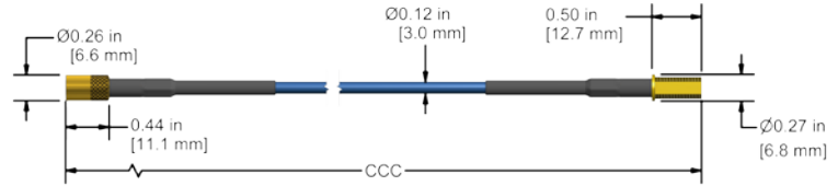
Armored Cable
