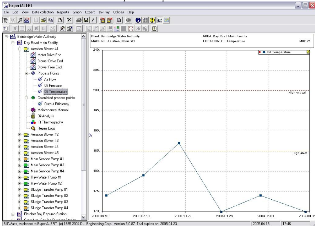
Fig. 3. Process point trend over time.
