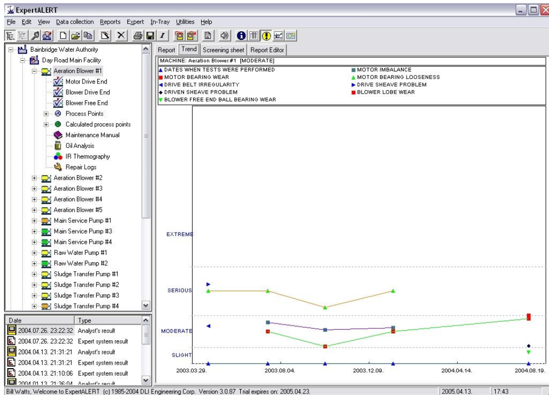
Fig. 2. Fault trend over time.
