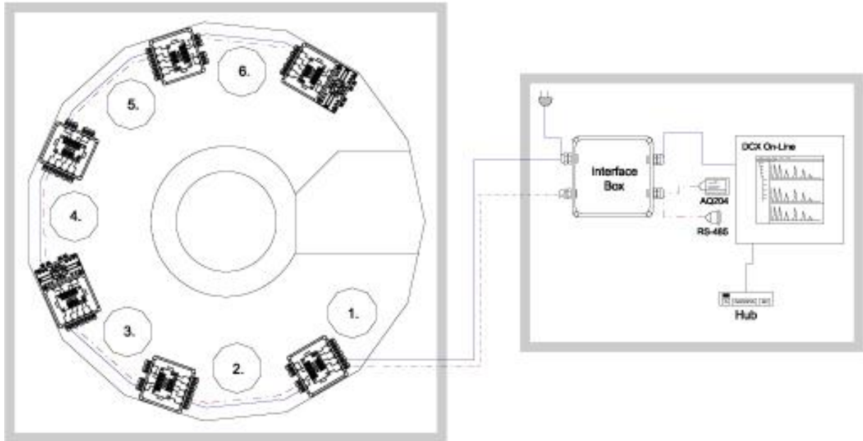
Fig. 5. Schema of on-line vibration diagnostic system at NPP Paks.
