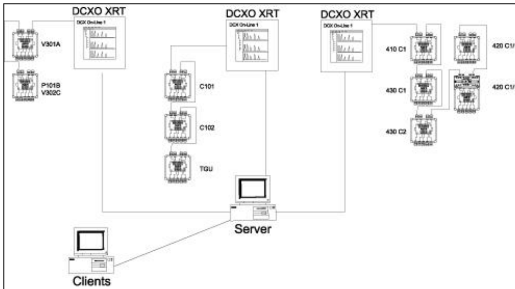
Fig. 6. Schema of on-line vibration diagnostic system at MOL Hungarian Oil and Gas Company
