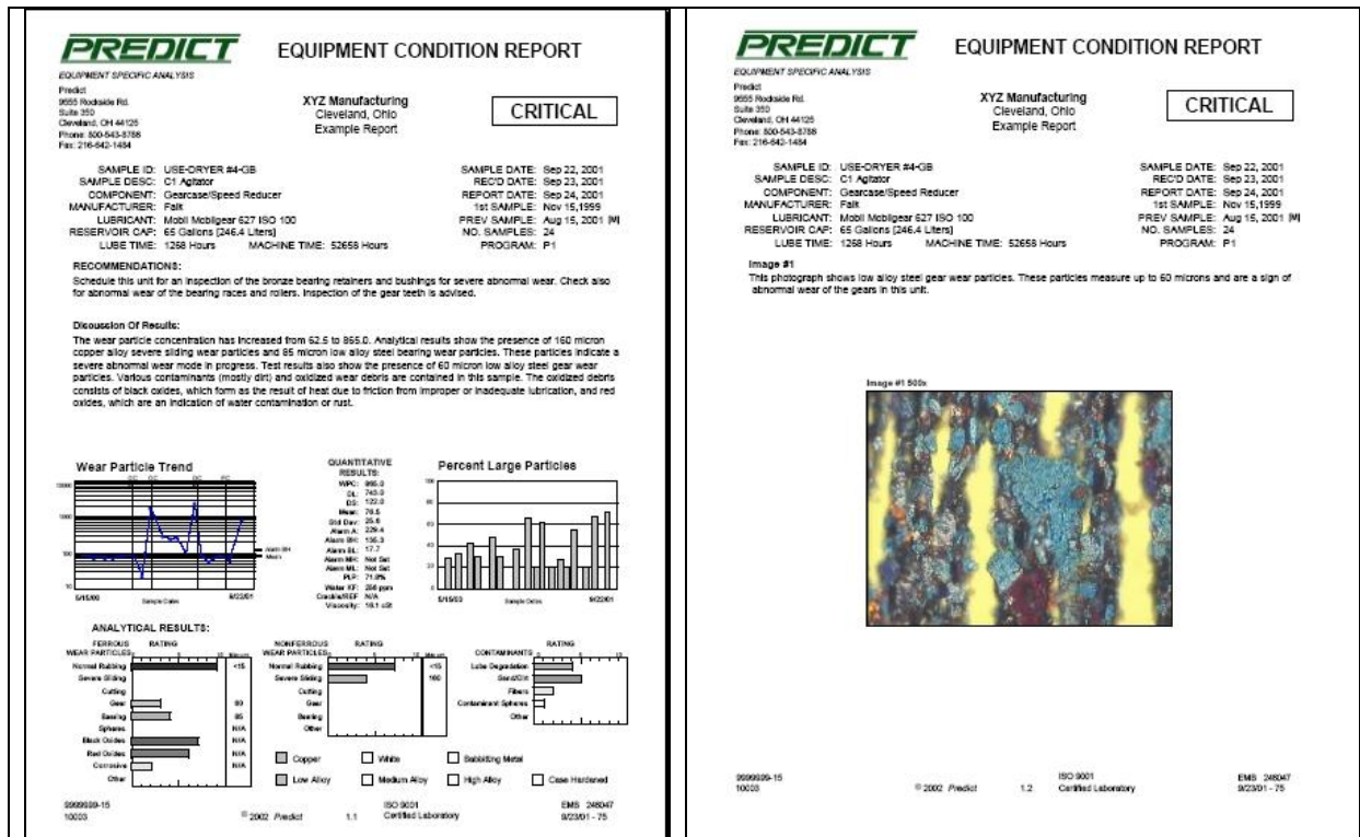
Fig 4. Oil Analysis and Ferrography report.
