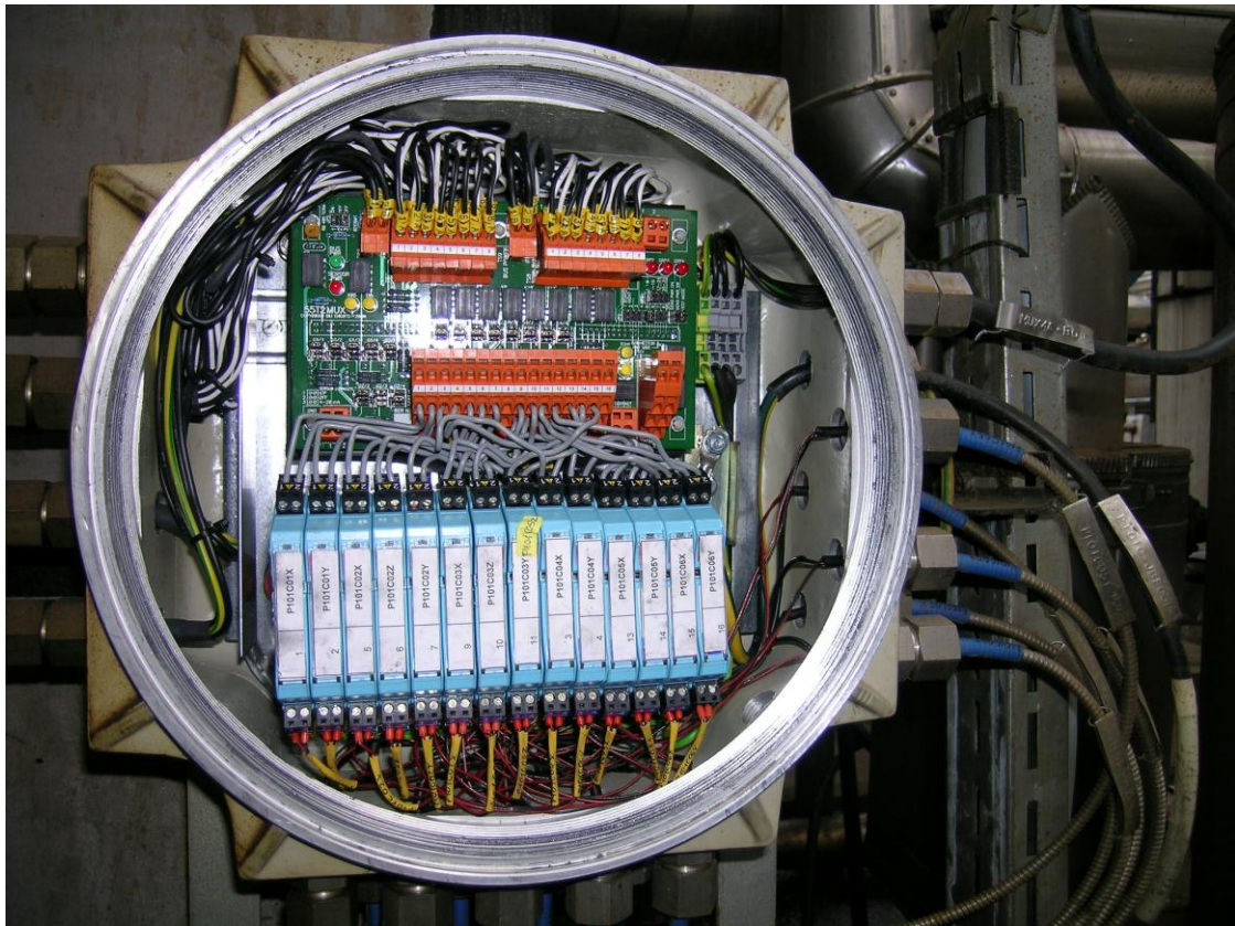
Figure 7. Explosion proof multiplexer unit
