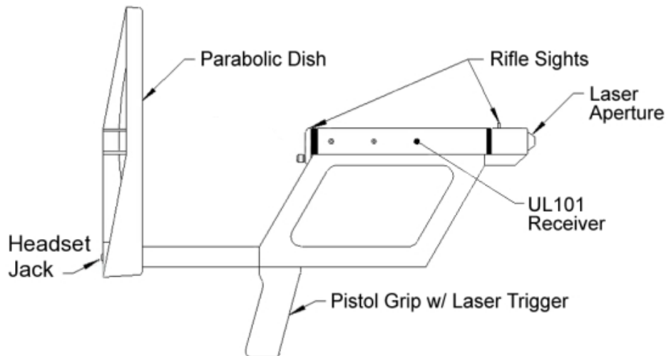
PowerBeam 300 Diagram
